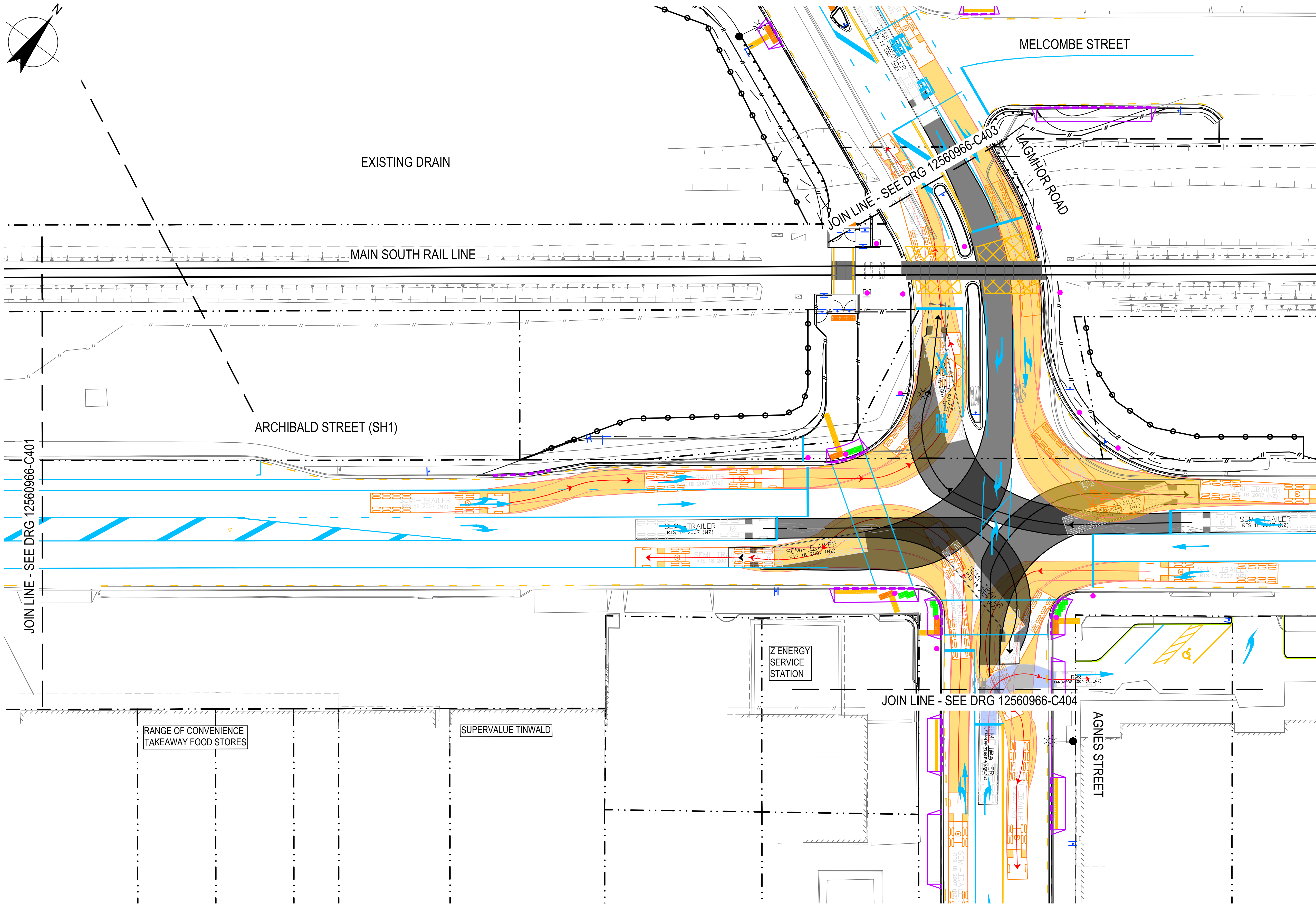
LAYOUT PLAN SCALE 1:250
