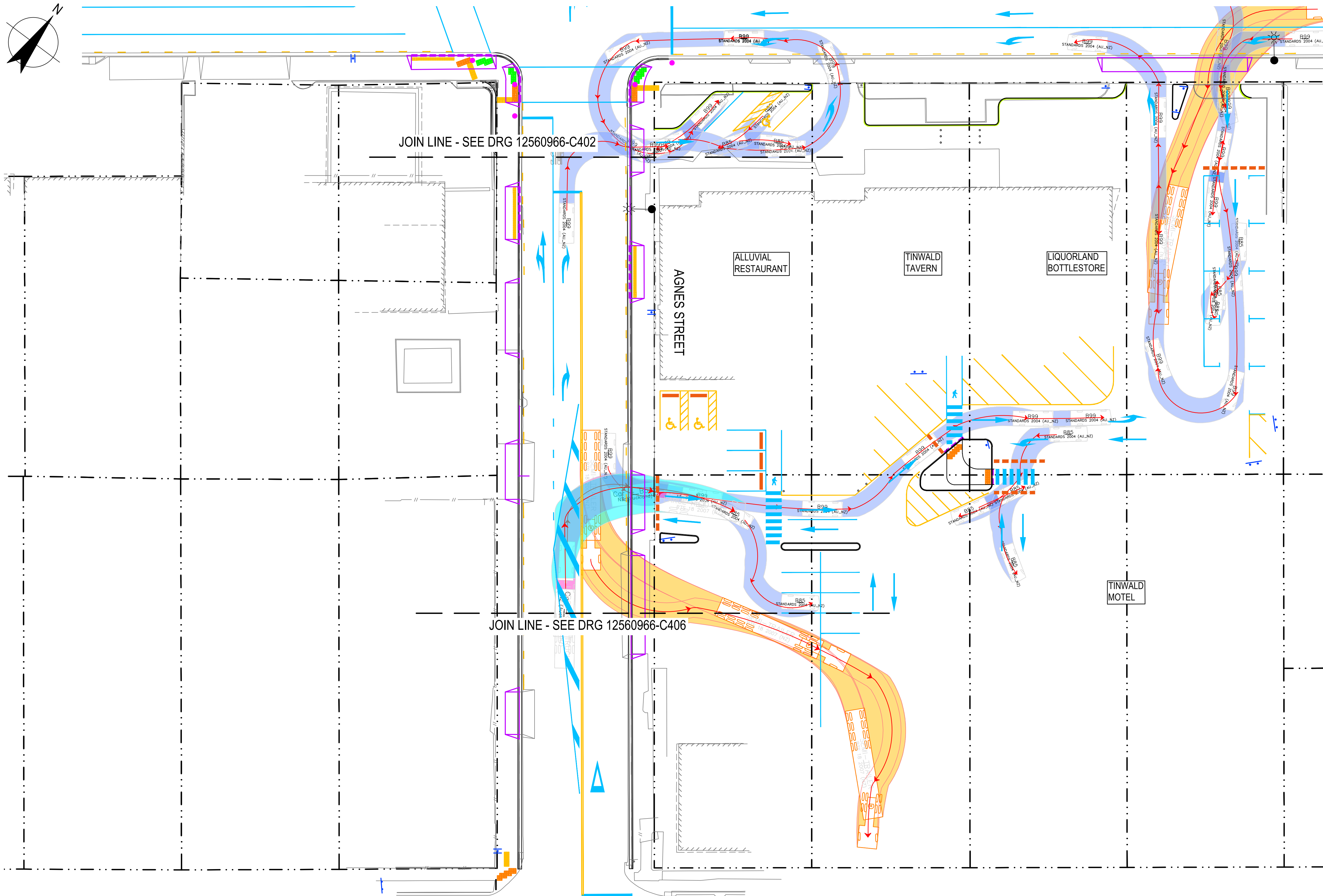
LAYOUT PLAN SCALE 1:250
